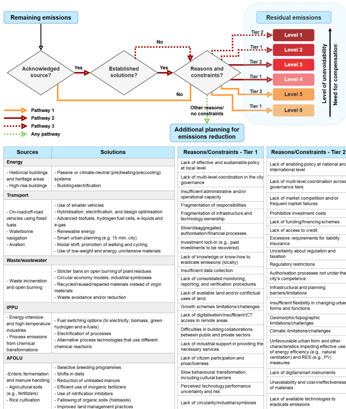
Figure 2. Schematisation of the conceptual framework to establish (qualitatively) the level of unavoidability of remaining emissions and thus distinguish remaining from residual emissions. AFOLU: agriculture, forestry, and other land use; ICT: information and communication technology; IPPU: industrial processes and product use; PV: photovoltaic; RES: renewable energy source.
