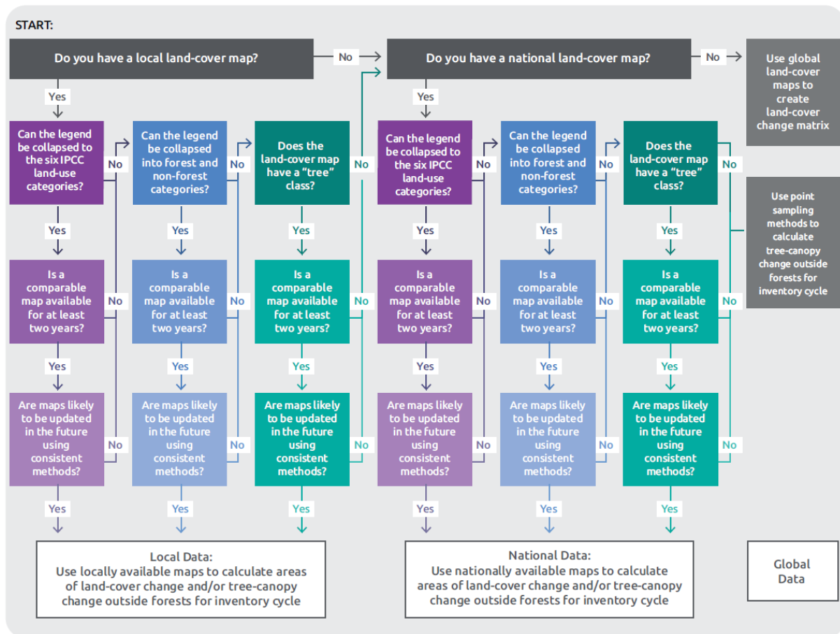
Figure 6. Decision tree for selecting sources of activity data.
