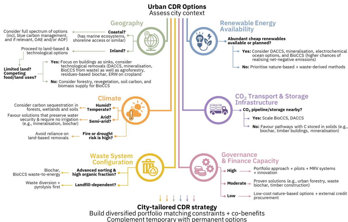
Figure 4. Decision tree for identifying urban carbon dioxide removal strategies tailored to a city's context. OAE: ocean alkalinity enhancement; AOF: artificial ocean fertilisation.
