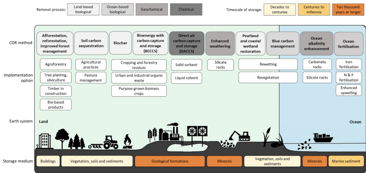
Figure 3. Carbon dioxide removal taxonomy. Methods are categorised based on removal process (grey shades) and storage medium (for which timescales of storage are given, yellow/brown shades). Main implementation options are included for each CDR method. Note that specific land-based implementation options can be associated with several CDR methods, for example, agroforestry can support soil carbon sequestration and provide biomass for biochar or BioCCS.
