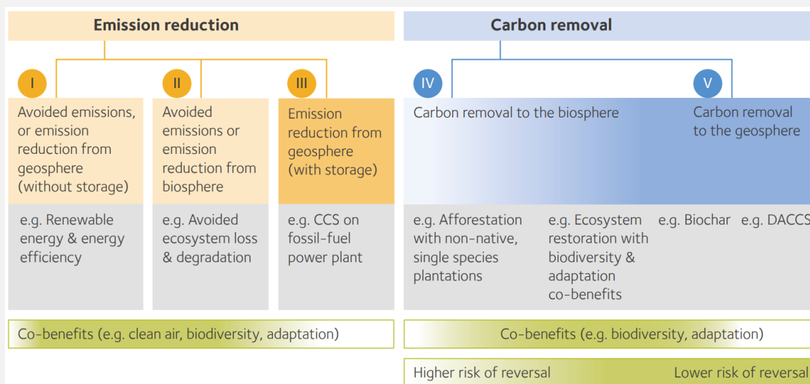
Figure 5. Simplified classification scheme of the five types of carbon offset. The shading of colours from light to dark pertain to the durability of storage. The risk of reversal of storage types and co-benefits are illustrated as gradient bars below the project types.
